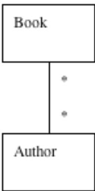
Class Diagram
