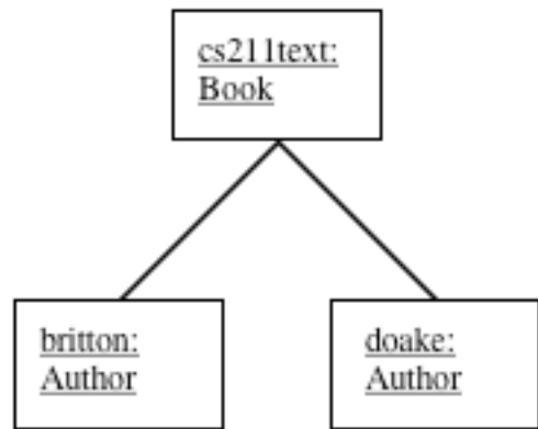
Object Diagram
